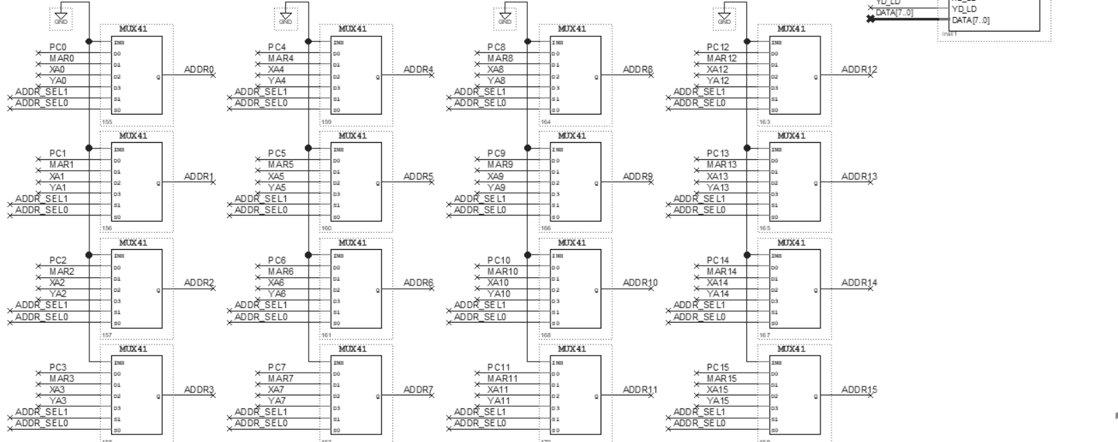
Address Selection/Generation
