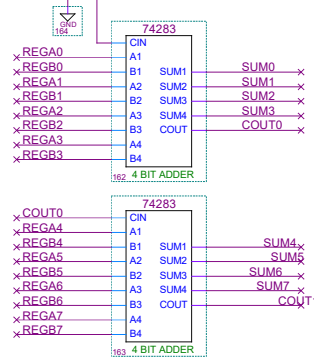
Sum & Carry Flag Generation
