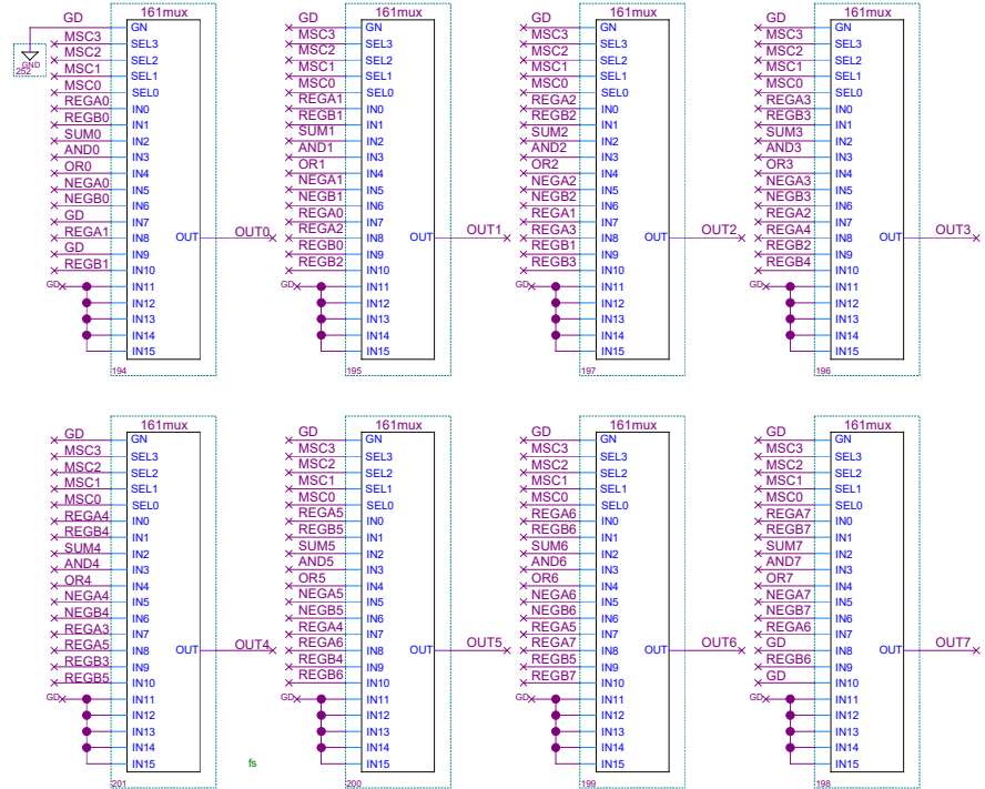
Mux C Block
