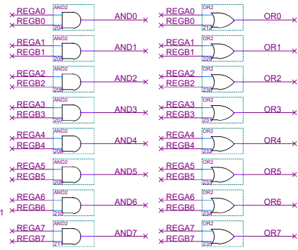
AND Generation
