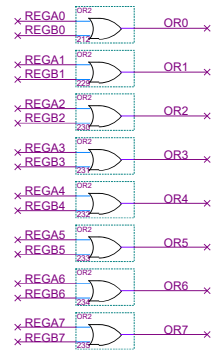
OR Generation
