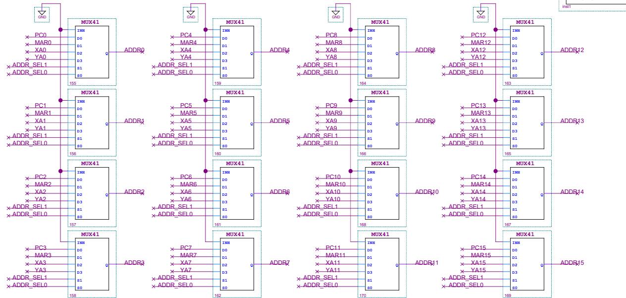
Address Selection/Generation
