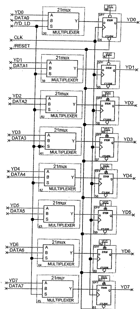
Y Displacement Register (YDR)
