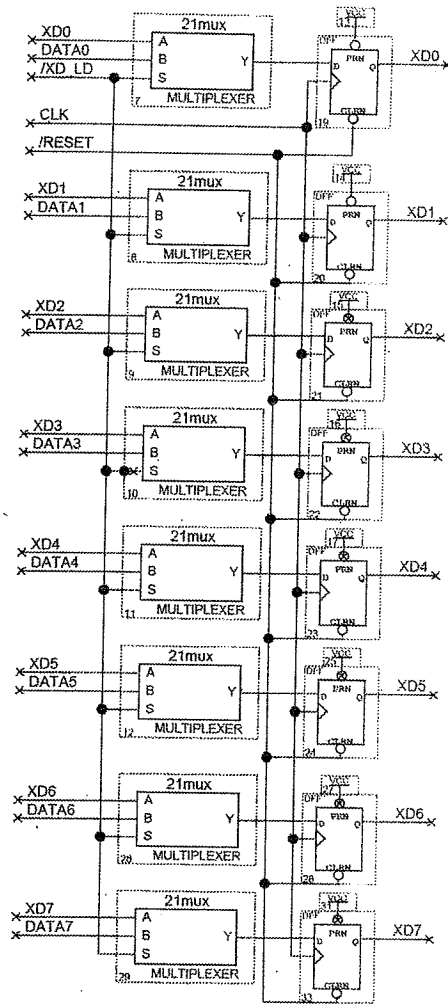
X Displacement Register (XDR)
