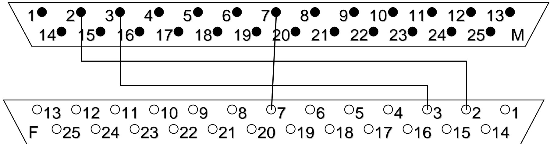
Male DB-25 (EVBU) to Female DB-25 (PC)
