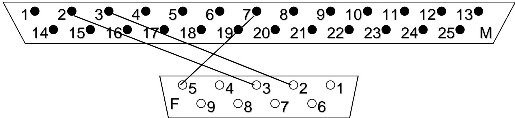
Male DB-25 (EVBU) to Female DB-9 (PC)
