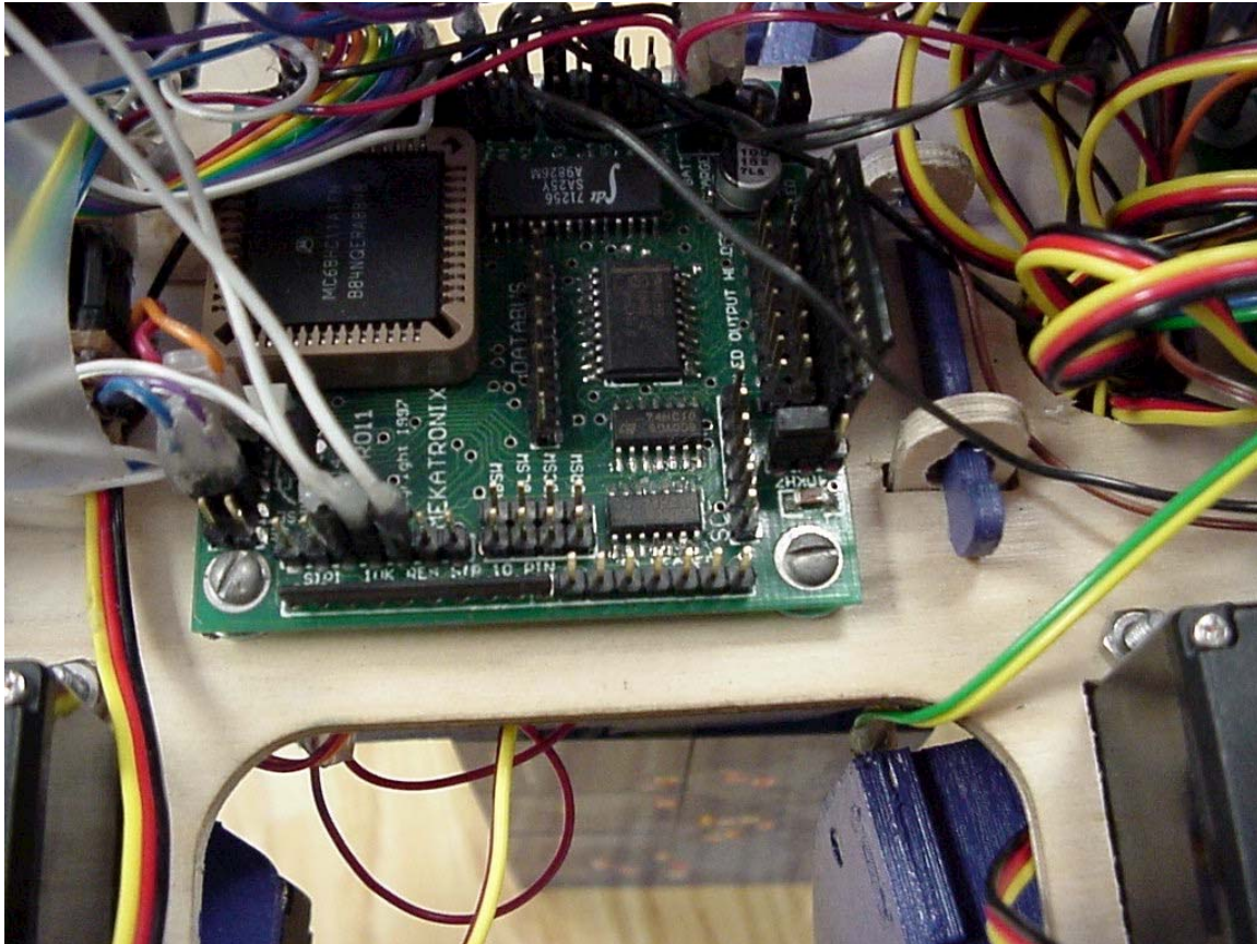
Figure 2. TJPro11 “brain board” with sensor, buzzer, LED, mode switch, and reset switch connected.
