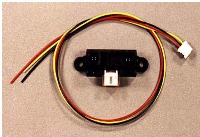
Figure 12. Picture of one of the Sharp GP2D12 Infrared Ranger's used in the height detection sensor.
