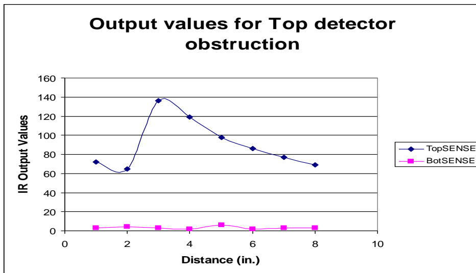
Figure 16. Output values for Top detector obstruction
