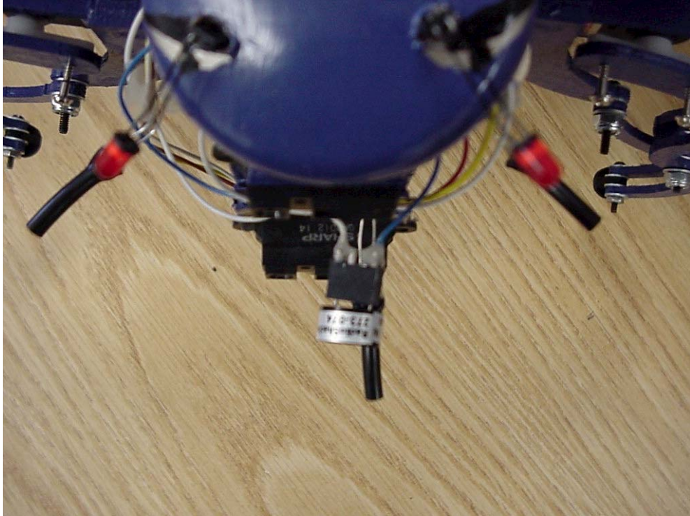
Figure 15. Photo of CdS sensor setup as seen from the top of the robot.. This photograph shows how the CdS sensors were arranged from left to right.
