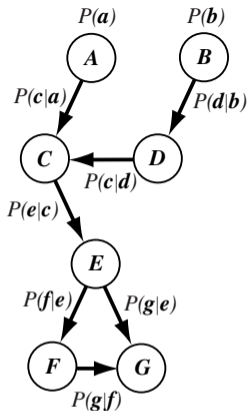
FIGURE 2.24. A belief network consists of nodes (labeled with uppercase bold letters) and their associated discrete states (in lowercase). Thus node A has states a_1, a_2, \dots , denoted simply \mathbf{a} ; node B has states b_1, b_2, \dots , denoted \mathbf{b} , and so forth. The links between nodes represent conditional probabilities. For example, P(\mathbf{c}|\mathbf{a}) can be described by a matrix whose entries are P(c_i|a_j) . From: Richard O. Duda, Peter E. Hart, and David G. Stork, Pattern Classification . Copyright © 2001 by John Wiley & Sons, Inc.
