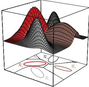
FIGURE 2.16. The decision regions for four normal distributions. Even with such a low number of categories, the shapes of the boundary regions can be rather complex. From: Richard O. Duda, Peter E. Hart, and David G. Stork, Pattern Classification . Copyright © 2001 by John Wiley & Sons, Inc.
