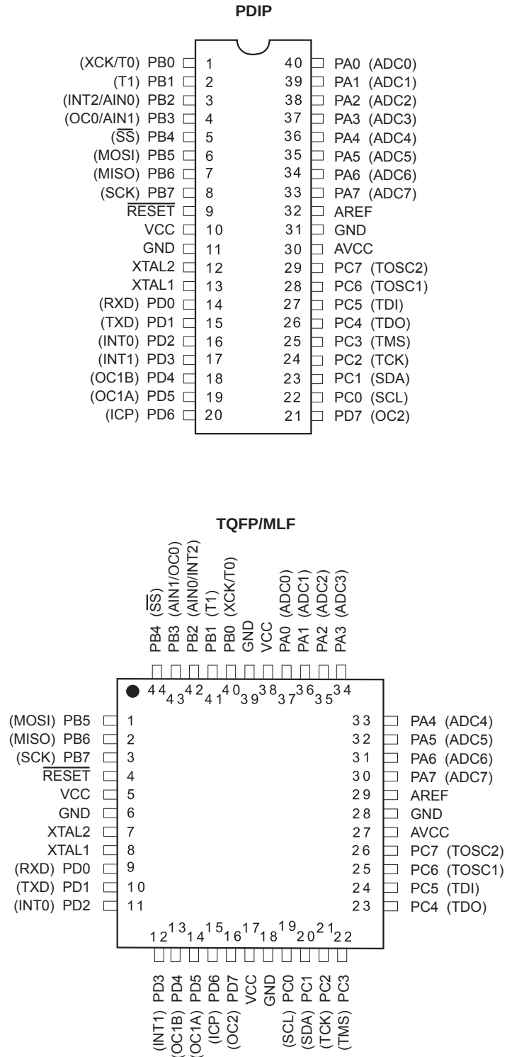
Figure 1. Pinouts ATmega32
