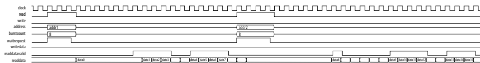
Figure 15. Incrementing Burst Read Operation for 10M50 Devices in Parallel Mode
