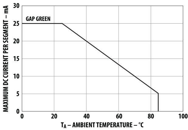
Figure 5. Maximum allowable average or DC current vs. ambient temperature.
