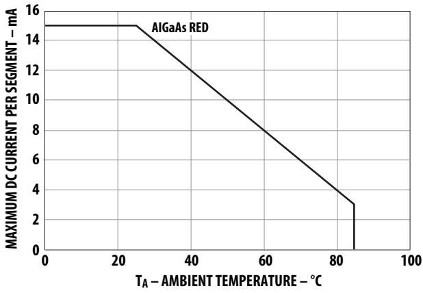
Figure 9. Maximum allowable average or DC current vs. ambient temperature.
