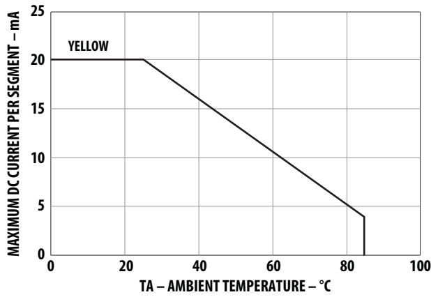
Figure 13. Maximum allowable average or DC current vs. ambient temperature.
