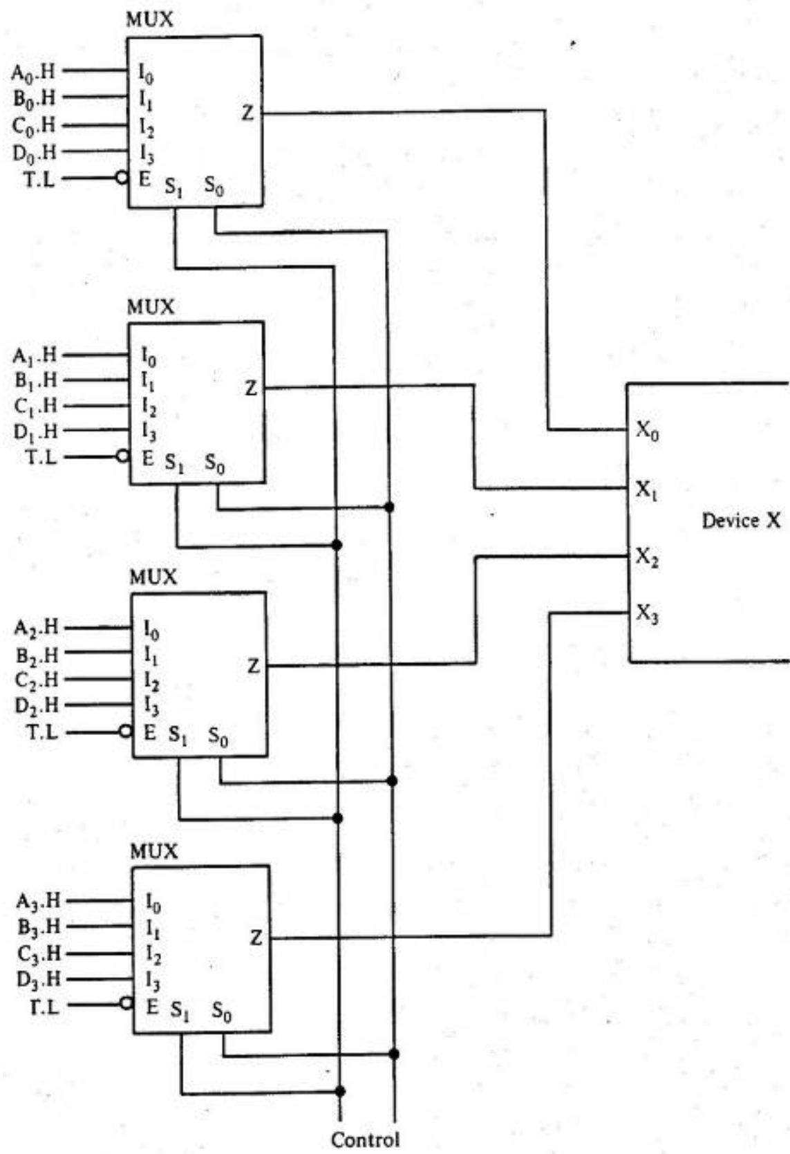
Figure 4.18 Using MUXs for data selection.
