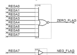
Z & N Flag Generation
