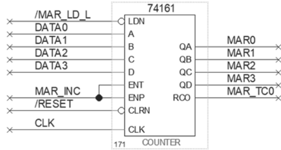
Memory Address Register
