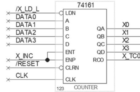
X Index Register
