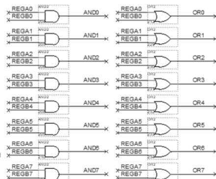
AND Generation
