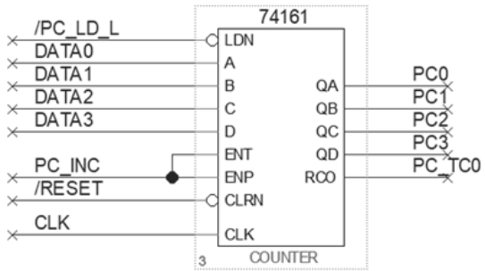
Program Counter Register
