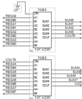
Sum & Carry Flag Generation
