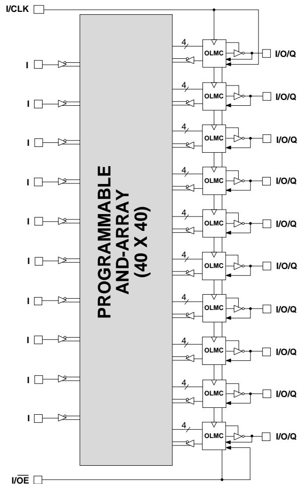
GAL20XV10 Block Diagram
