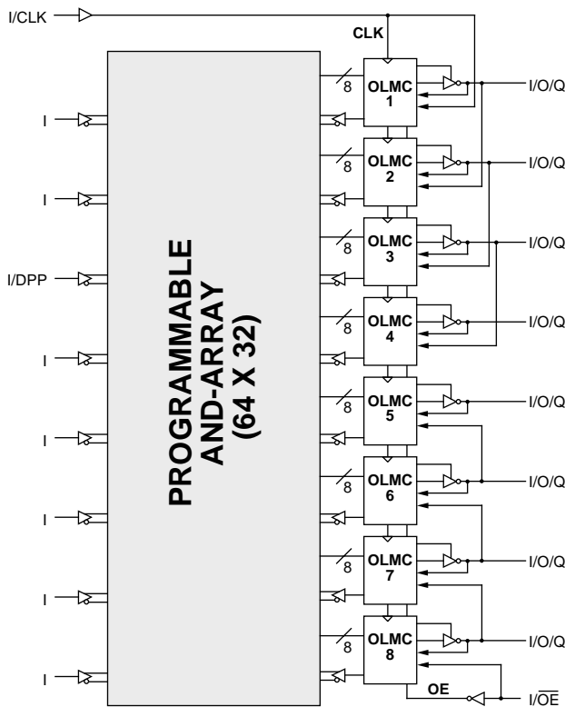
GAL16V8Z/ZD Block Diagram
