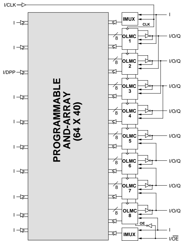
GAL20V8Z/ZD Block Diagram
