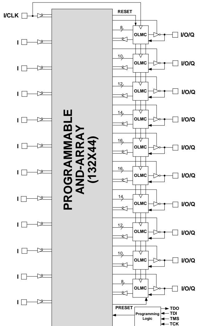
ispGAL22LV10 Block Diagram
