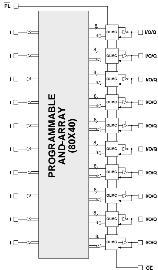
GAL20RA10 Block Diagram
