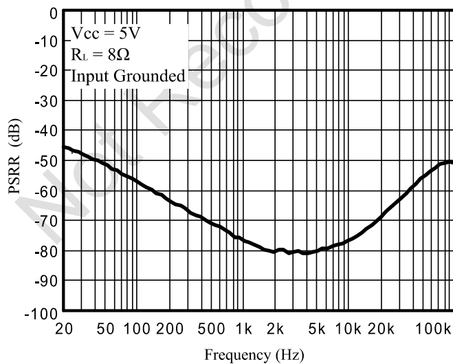
Figure 7 PSRR vs. Frequency
