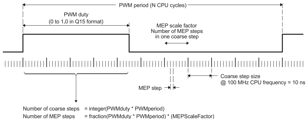
Figure 2. Operating Logic Using MEP
