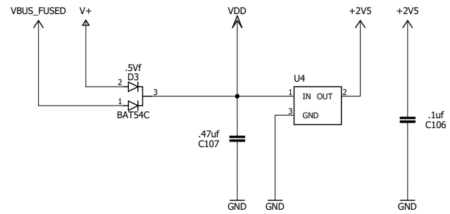
2.5V Analog Reference
