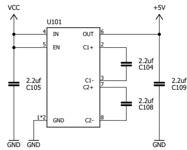
5.0V Buck Boost Regulator
