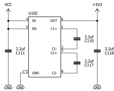
3.3V Buck Boost Regulator
