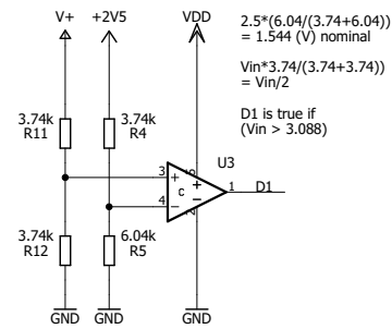
Comparator for Undervoltage Lockout
