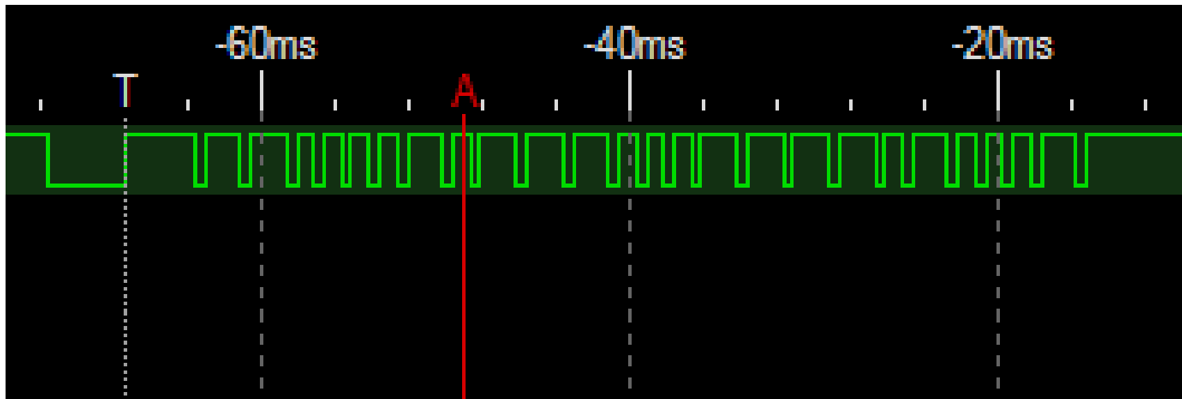
LSA capture of IR signals from an RCA TV remote controller
