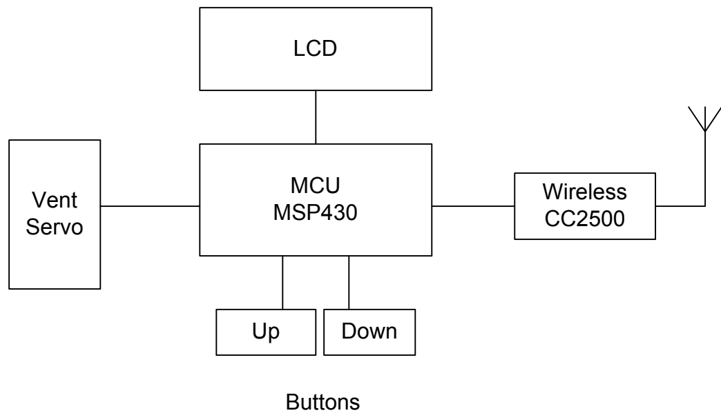
Individual Room Controller (IRC)
