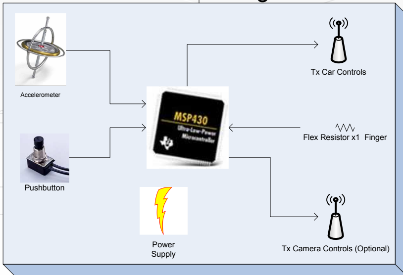
Glove Block Diagram
