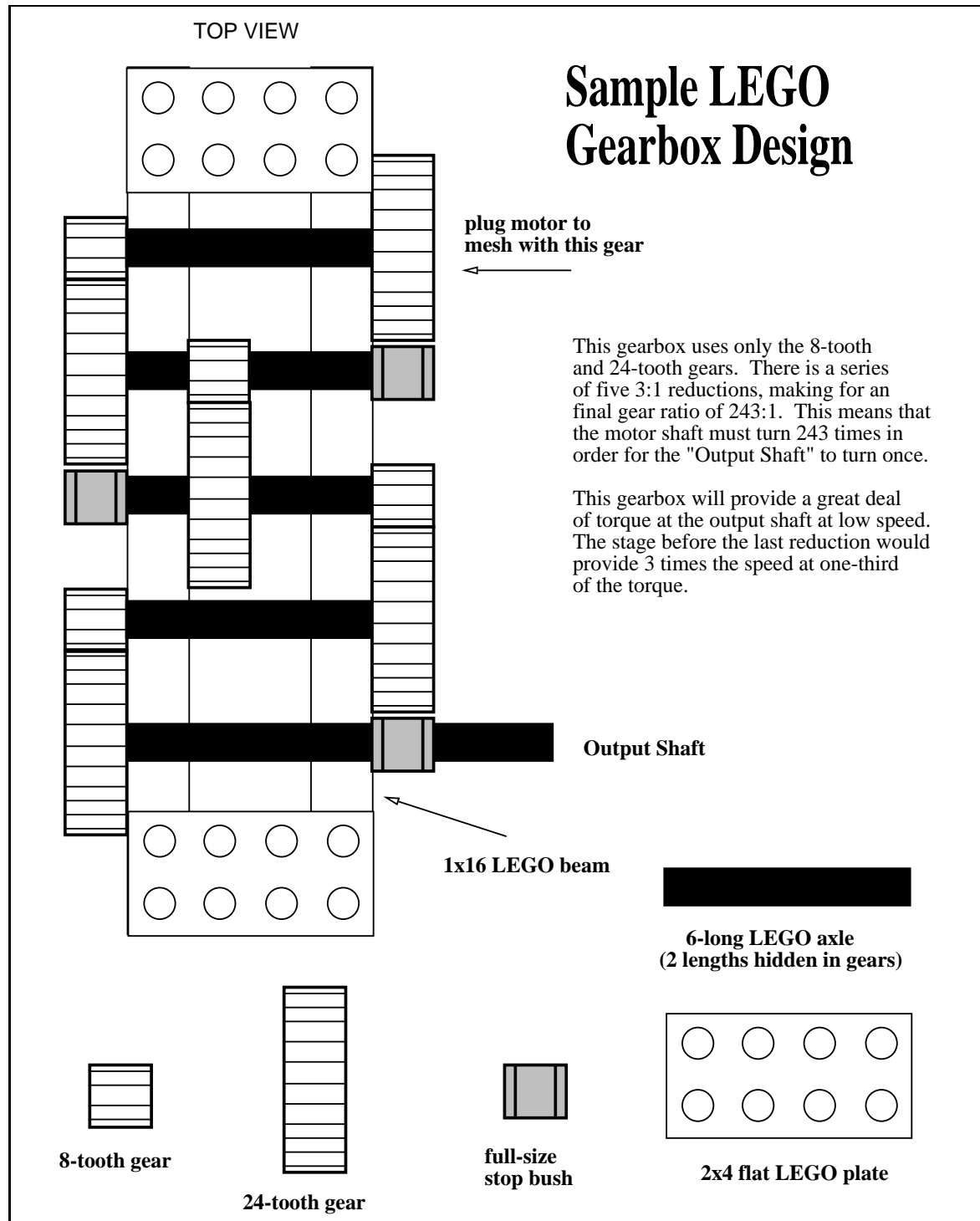
Figure 7.7: LEGO Gearbox Example
