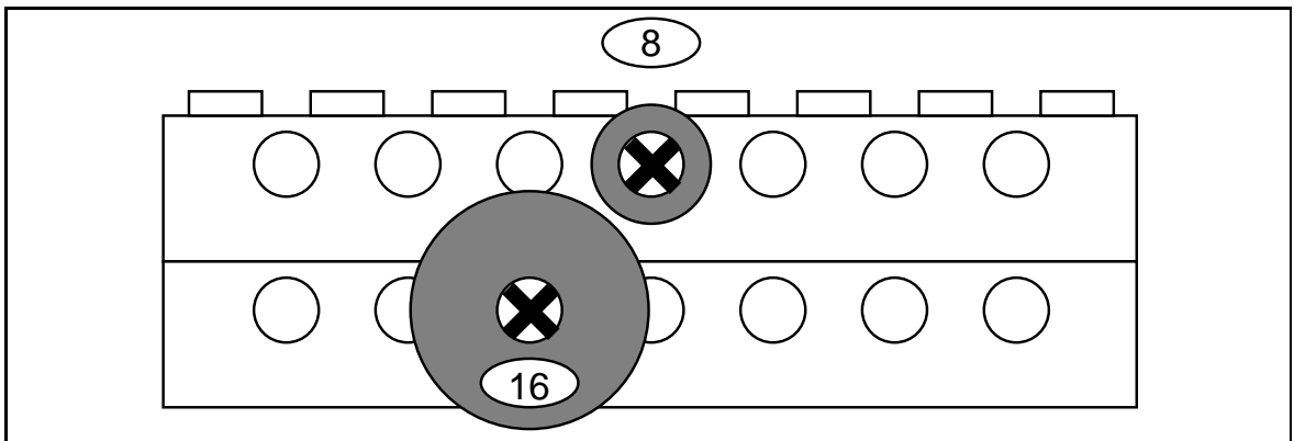
Figure 7.5: Diagonal Meshing of an 8-Tooth Gear and a 16-Tooth Gear
